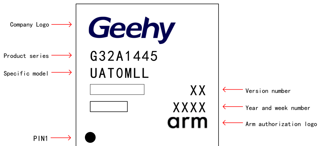
Figure 26 LQFP100 - 100 Pins, 14 x 14mm Diagram
