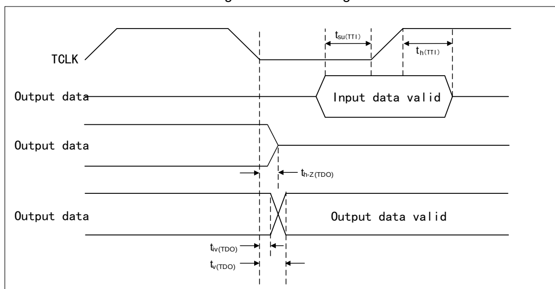
Figure 23 TDO Timing
