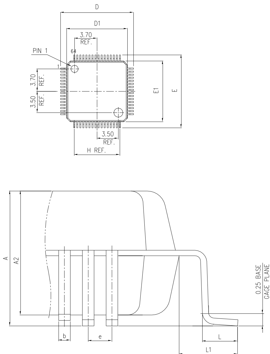
Figure 27 LQFP64 Package Diagram
