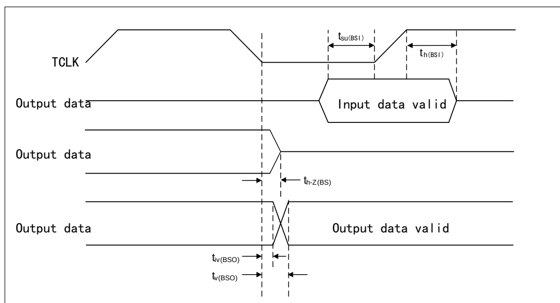
Figure 22 JTAG Boundary Scan Timing
